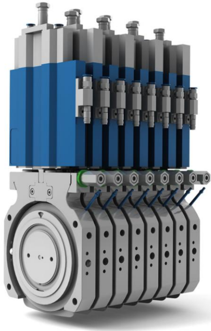
Clever: Nested knife holder for narrowest slitting widths DIENES Knife holder DS 4
